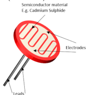
Fig 3. parts of an LDR
